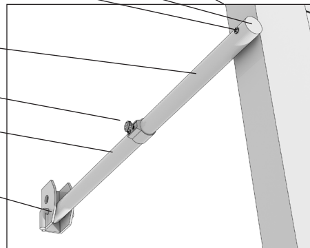
SL Bahama Arm Cap S-60-00-00102 SL 2" Sidewalk Bolt Stainless Steel S-60-00-00124 SL Bahama Arm Bushing S-60-00-00117 SL Bahama Arm 1" 20' S-60-63-00021 SL 1" Anti Seize Collar S-60-00-00104 SL Bahama Arm 7/8 20' S-60-63-00020 SL Camel Back w/Pin S-60-00-00105
