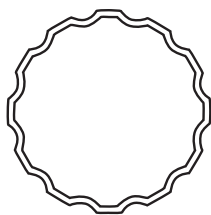
11771 Fluted Round Tube Size Size. 5 X 3/16 (.188) Length. Ft. 24 Wt. Lin Ft. 3.524
