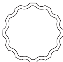
11722 Fluted Round Tube Size. 3 X .125 Length. Ft. 24 Wt. Lin Ft. 1.404
