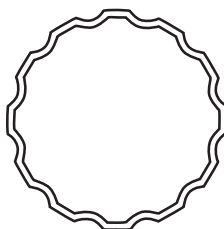
11786 Fluted Round Tube Size. 6 X .250 Length. Ft. 24 Wt. Lin Ft. 5.504
