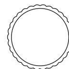
14046 Serrated Awning Tube Size. 1 X .049 Length. Ft. 24 Wt. Lin Ft. .152
