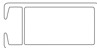
14010 Size: 1 X 2 X .093 Wt. Lin. Ft. .603
